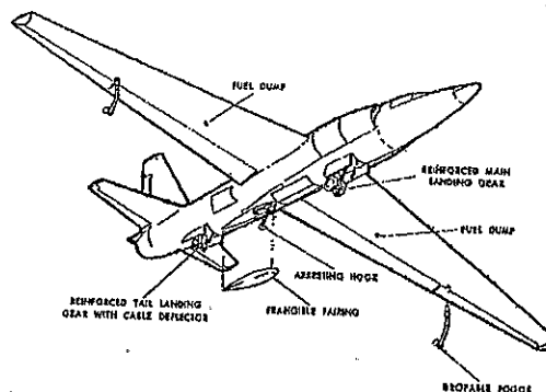
DESIGN PROPOSALS for developing a U-2 with a carrier launch capability were submitted as early as 1957, as shown here. The configuration ultimately chosen most nearly resembles that in the lower drawing with the addition of some additional features such as the mechanical spoilers installed on the wings.
